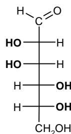
D-mannosio
