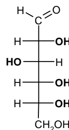
D-glucosio
